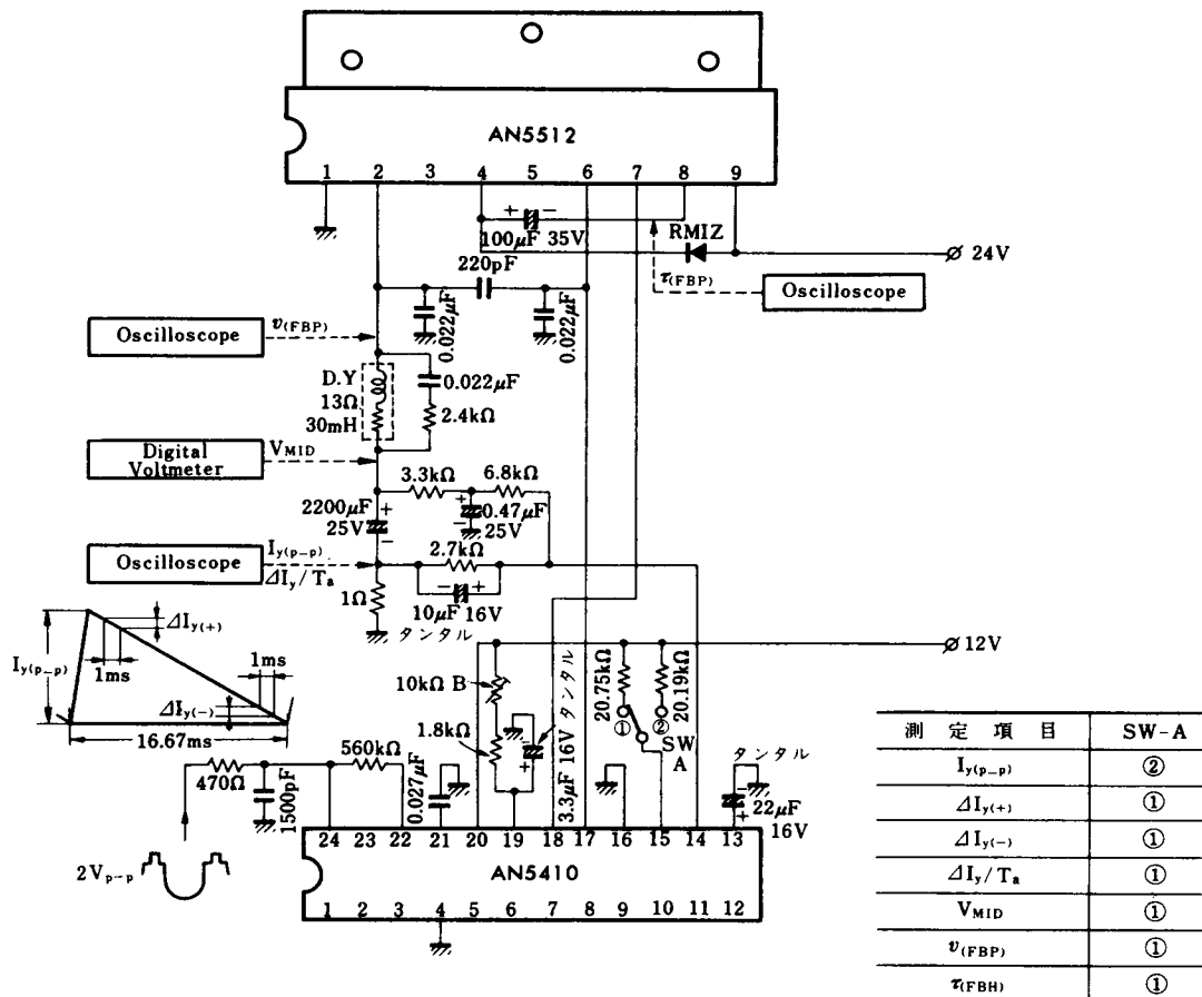
Test Circuit 1 ( I_{y(p-p)} , \Delta I_{y(+)} , \Delta I_{y(-)} , \Delta I_y/T_a , V_{MID} , v_{(FBP)} , \tau_{(FBP)} )
